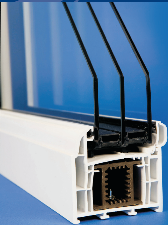
B07 70mm Outerframe Profile Shown
