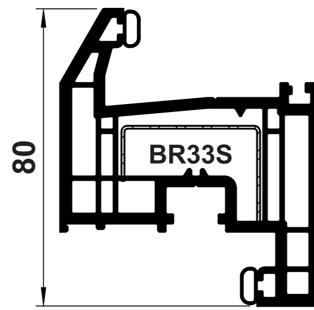
B33 TILT & TURN SASH
