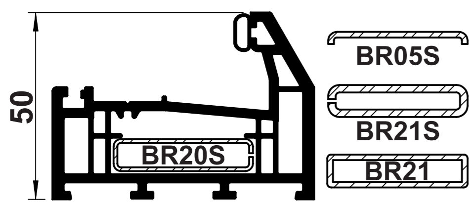
B01 OUTER FRAME
