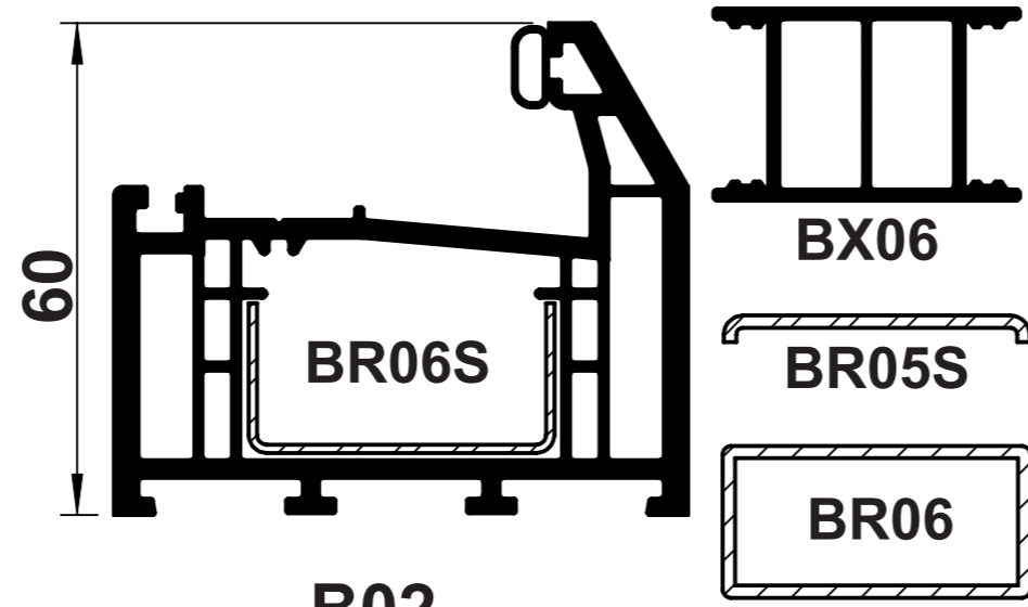
B02 OUTER FRAME
