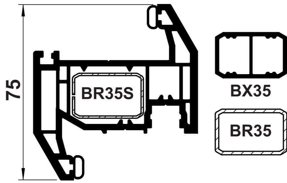
B31 CASEMENT 'Z' SASH
